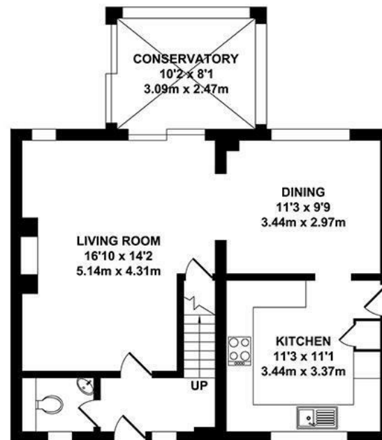
GROUND FLOOR APPROX. FLOOR AREA 638 SQ.FT. (59.27 SQ.M.)
