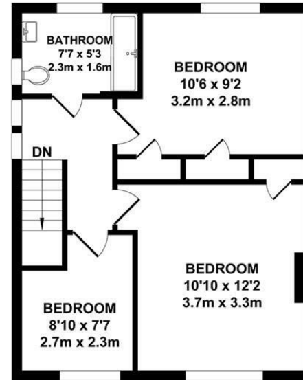
FIRST FLOOR APPROX. FLOOR AREA 428 SQ. FT. (39.76 SQ. M)
