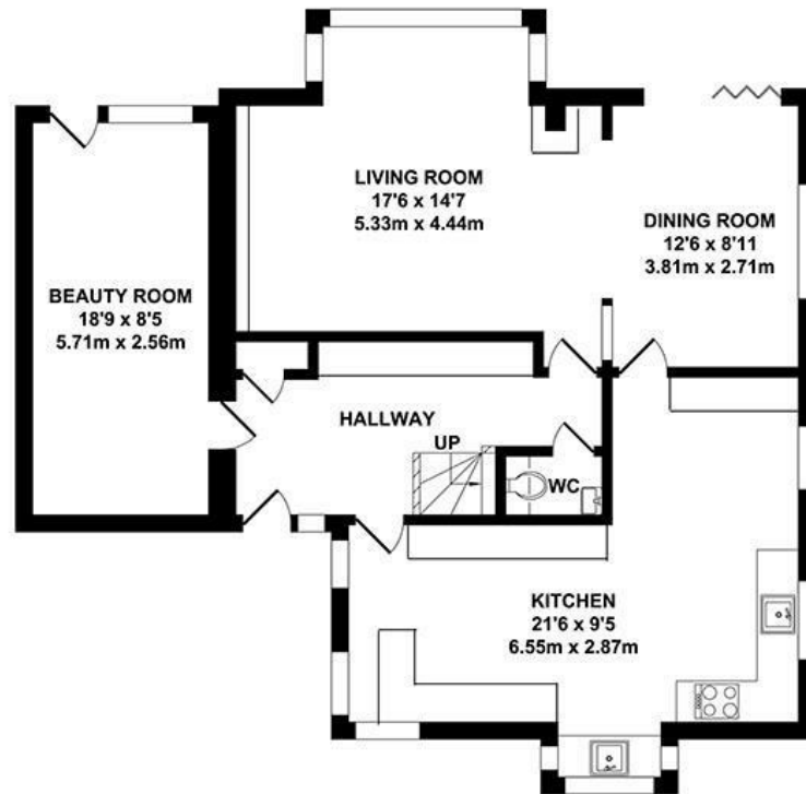
GROUND FLOOR APPROX. FLOOR AREA 970 SQ.FT. (90.14 SQ.M.)
