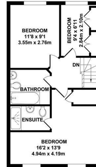
SECOND FLOOR APPROX. FLOOR AREA 480 SQ.FT. (44.62 SQ.M.)
