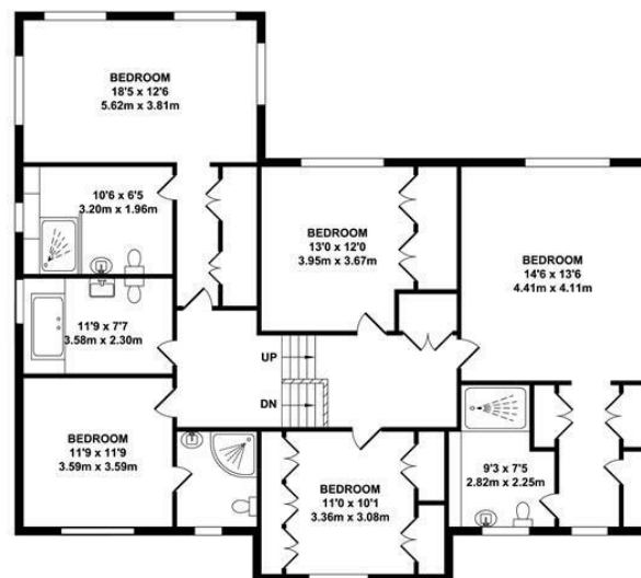
FIRST FLOOR APPROX. FLOOR AREA 1663 SQ.FT. (154.46 SQ.M.)
