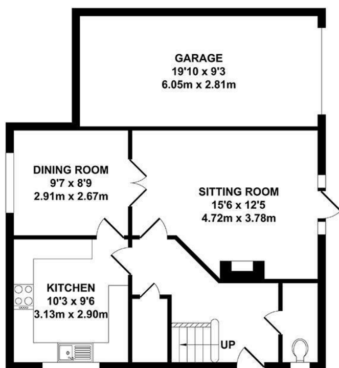
GROUND FLOOR APPROX. FLOOR AREA 680 SQ.FT. (63.21 SQ.M.)
