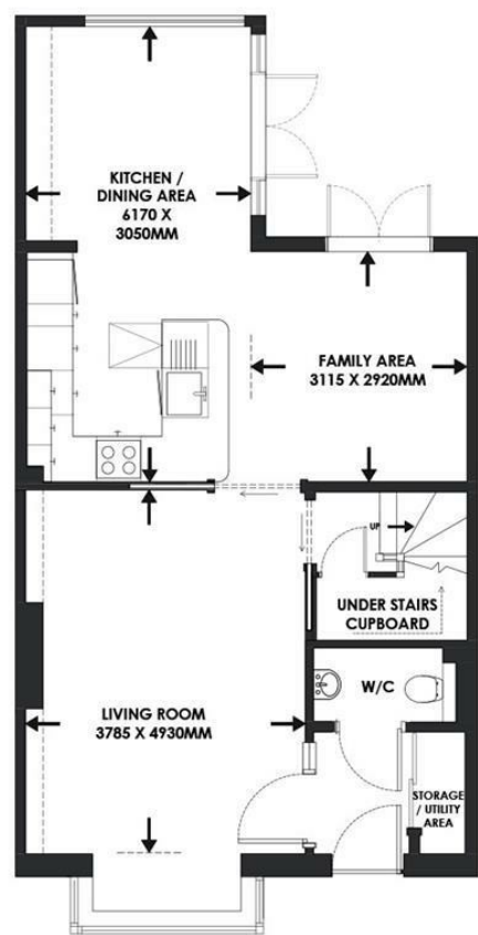
GROUND FLOOR APPROX FLOOR AREA 645 SQ FT (60M2)
