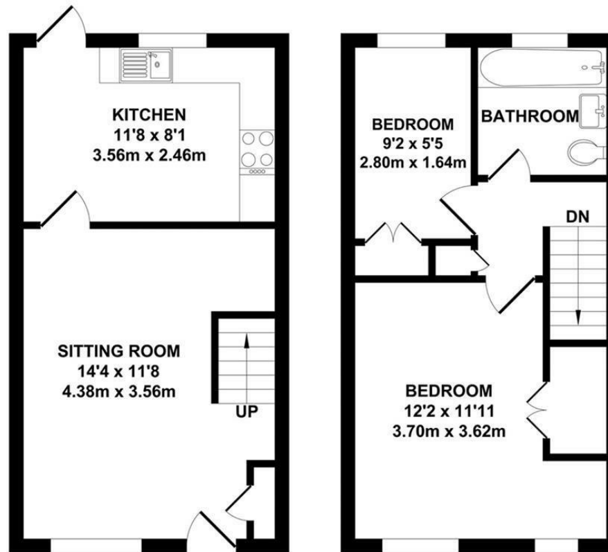
GROUND FLOOR APPROX. FLOOR AREA 266 SQ. FT. (24.71 SQ. M)
